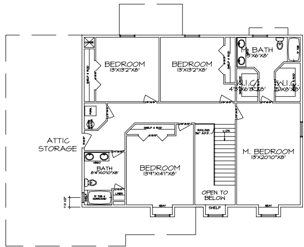
1 SECOND FLOOR PLAN A-5 SCALE: 1/4"=1'-0"
