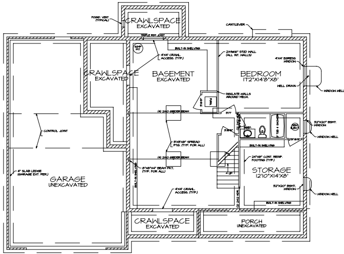
1 FOUNDATION PLAN A-3 SCALE: 1/4"=1'-0"
